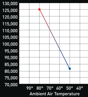
Heating BTU Rating per Hour UltraTemp 120 & 120 R/H/C
