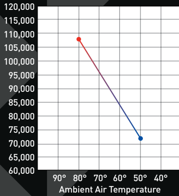
Heating BTU Rating per Hour UltraTemp 110
