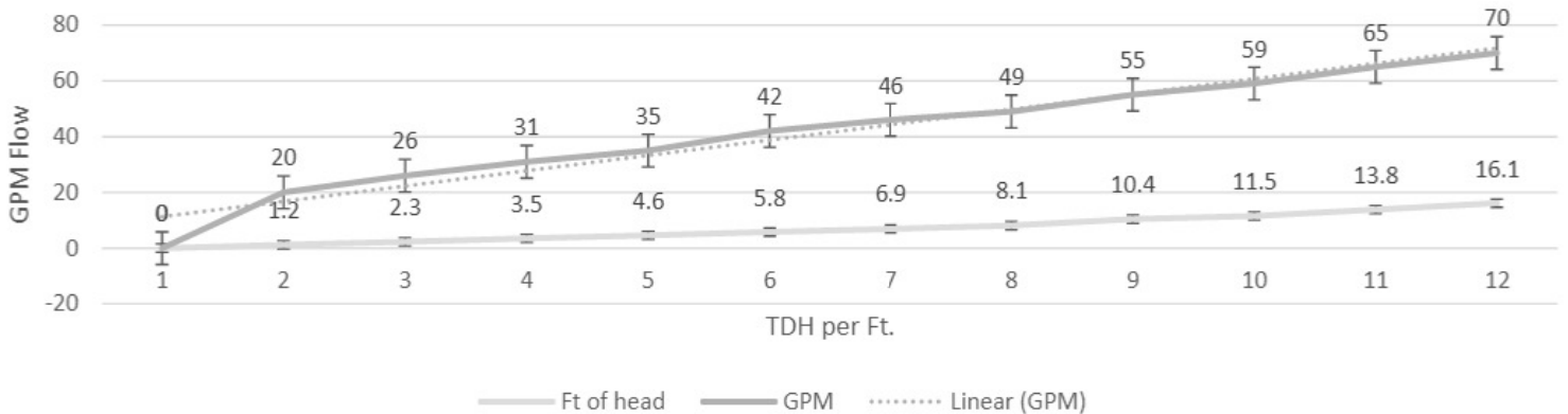
Head Loss
