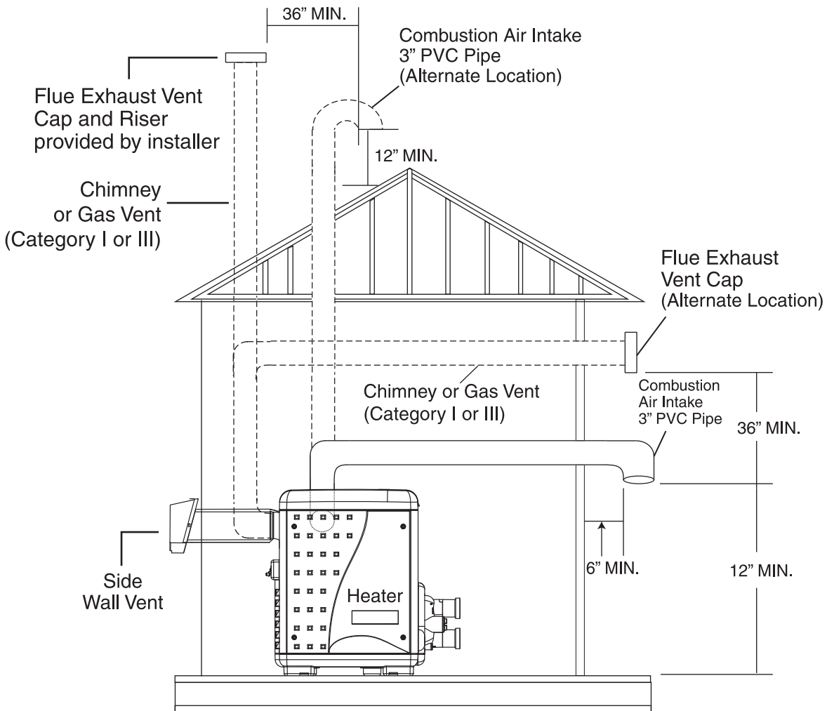
Direct Air Intake Duct with 3-inch PVC Pipe (Indoor Installation) (MasterTemp® Heater shown)
